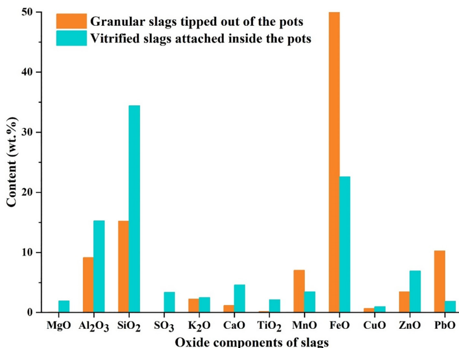
Fig. 10. Comparison of the mean oxide contents in the granular slags tipped out from the pots and the vitrified slags attached inside the pots.
