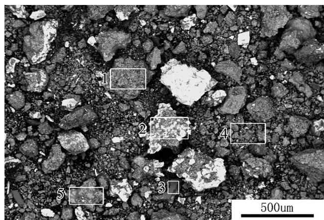
Fig. 8. Backscattered electron image of zinc calcine (DZC-1). The white particles are cerussite and anglesite, and some cerussite and anglesite particles are embedded in the franklinite.
