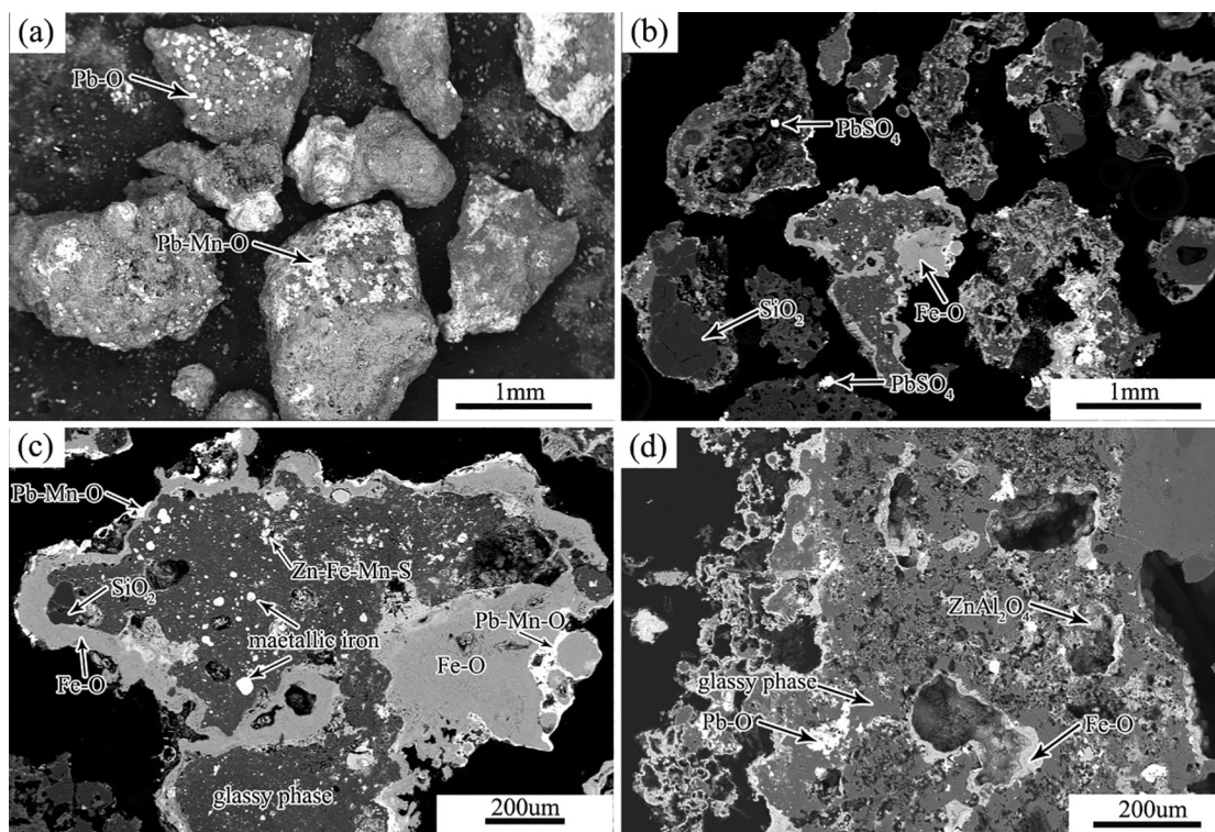
Fig. 11. Backscattered electron images of the zinc smelting slags: (a) granular slags tipped out from the pots with the lead-rich phases on the particle surface; (b) cross-section of the granular slags; (c) a trace amount of metallic iron prills and Zn-Fe-Mn-S mineral grains found in a vitrified particle; (d) slags attached in the bottom of the pot with a vitrified substrate.
