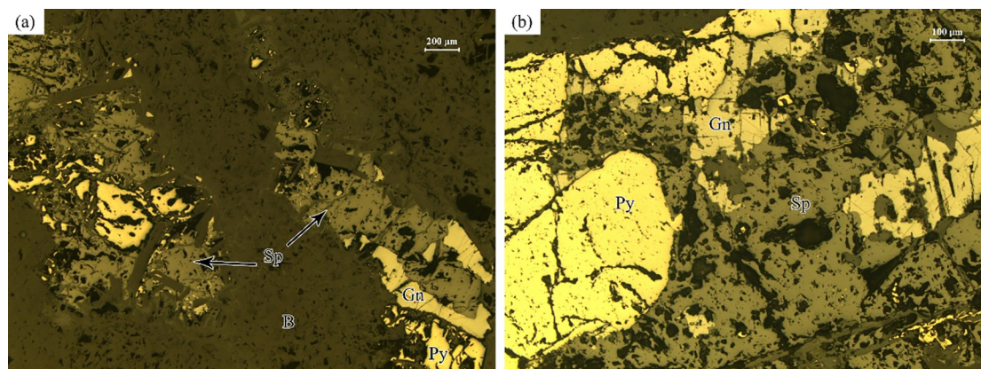
Fig. 3. The single polarized images of the ore TM04: (a) Sphalerite (Sp), galena (Gn), and pyrite (Py) are disseminated in an embedded substrate composed of non-metallic minerals (B); (b) Sphalerite and galena are intergrowth and distributed along the edge of pyrite.
