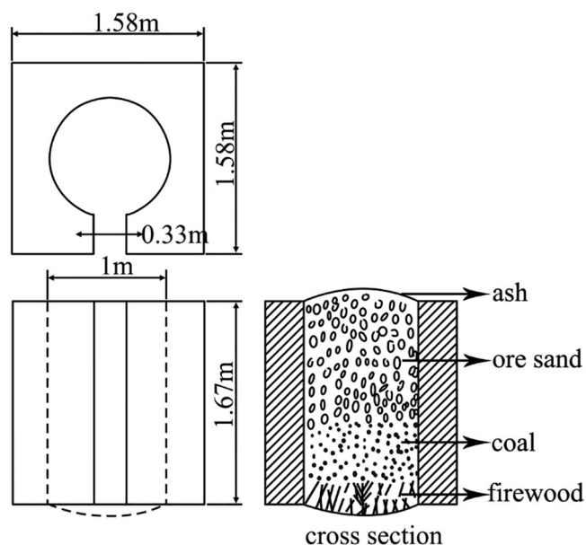
Fig. 14. Schematic diagram of the roasting hearth in the Songbai Traditional Zinc Smelting Plant in the 1930s (Zhou, 1930).
