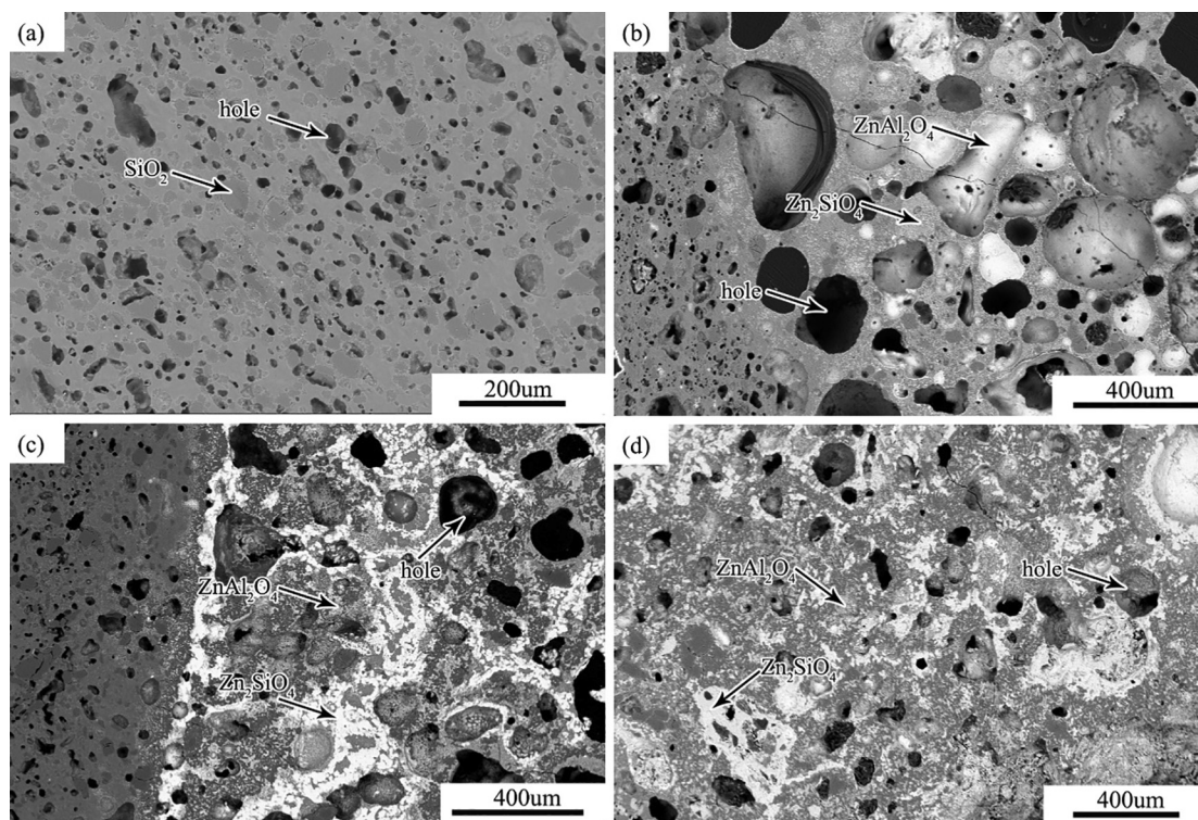
Fig. 5. Backscattered electron images of (a) unused pot TP02; (b) clay wrap on the outside of the used pot TP4; (c) interface between the rim of pot (left) and condenser (right); (d) residual pocket at the lower end of the crude zinc block.
