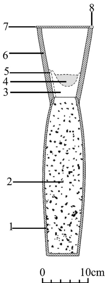
Fig. 12. Reconstruction of a retort (1-pot, 2-reaction ingredients, 3-pocket, 4-liquid zinc, 5-airway, 6-condenser, 7-lid, 8-exhaust hole).
