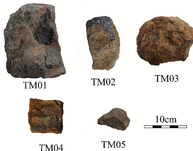
Fig. 2. The ores unearthed in the Tongmuling site.
