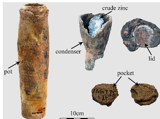
Fig. 4. The remains related to the retorts unearthed in the Tongmuling site.
