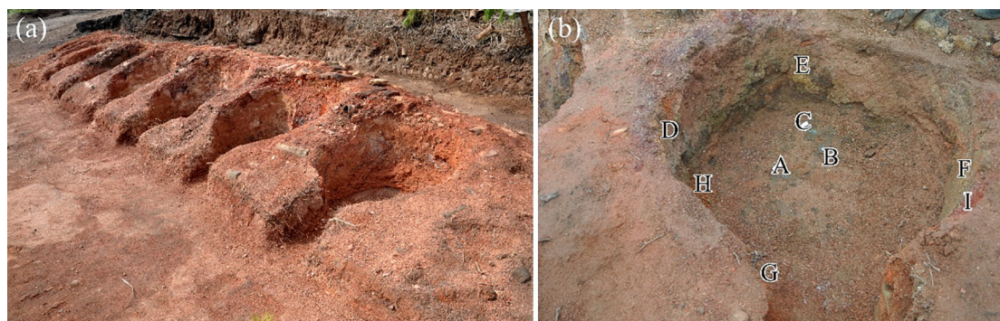
Fig. 6. The Cylindrical roasting hearths excavated in the Tongmuling site: (a) one of roasting platforms; (b) testing points of p-XRF analyses.
