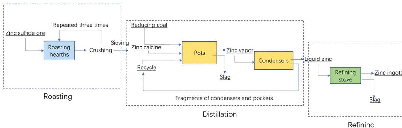
Fig. 13. Reconstruction of the distillation process of zinc sulfide ores in the Tongmuling site.
