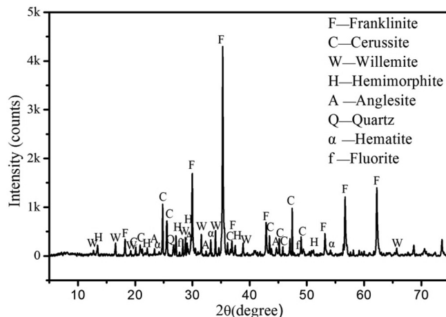
Fig. 7. XRD patterns of the zinc calcine (DZC-1) showing that the main phases include franklinite, cerussite, willemite, hemimorphite, and a small amount of anglesite, quartz, hematite and fluorite.
