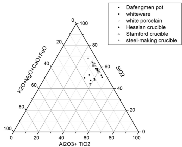
Fig. 8. Ternary diagram of SiO 2 –(Al 2 O 3 + TiO 2 )–(K 2 O + MgO + CaO + FeO) showing the matrix compositions of the Dafengmen pots and some kaolinitic ceramics: Neolithic and Shang whitewares (Kerr and Wood, 2004), Ding white porcelains (Kerr and Wood, 2004), Hessian crucibles (Martinón-Torres and Rehren, 2009), Stamford crucibles (Freestone and Tite, 1986) and Central Asian steel-making crucibles (Rehren and Papachristou, 2003).
