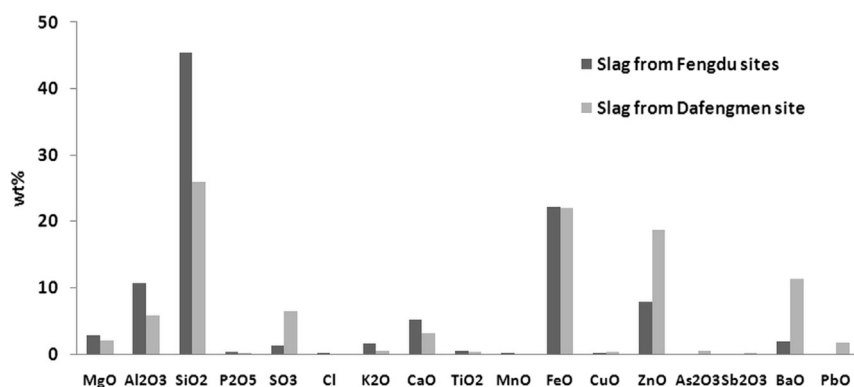
Fig. 9. Bar chart comparing average bulk compositions of the slag samples from the Fengdu sites and Dafengmen.
