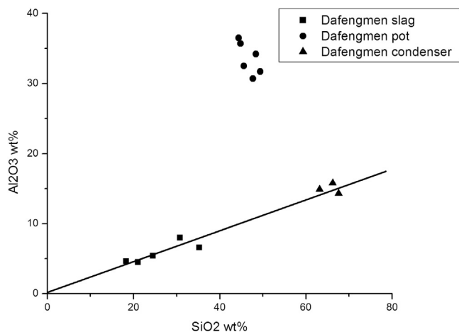
Fig. 10. The SiO 2 and Al 2 O 3 contents in the slag, pot and condenser samples from Dafengmen. Note the linear correlation of the SiO 2 and Al 2 O 3 contents of the slag and condenser samples.
