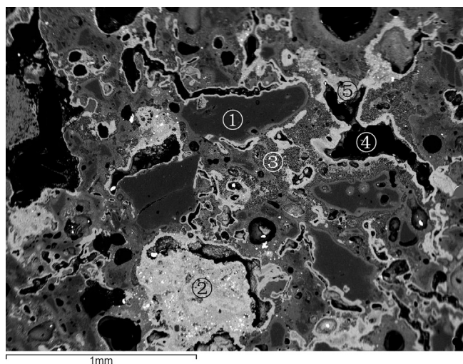
Fig. 3. BSE image of the pot fabric of SDT13, including rock fragments (1), ferruginous concretions (2), silica (3), pores (4) and the zinc-rich layers (5) lining the pores.
