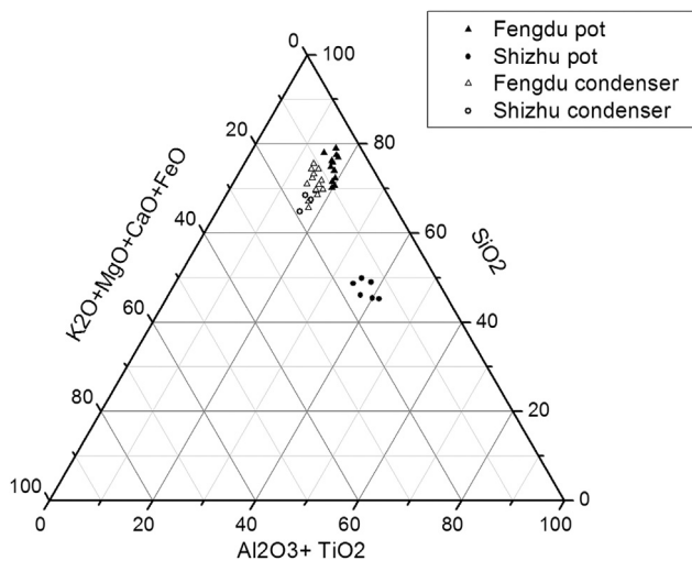
Fig. 7. Ternary diagram of SiO 2 –(Al 2 O 3 + TiO 2 )–(K 2 O + MgO + CaO + FeO) showing the bulk compositions of the pot and condenser fabrics from Fengdu (three sites) and Shizhu (Dafengmen).
