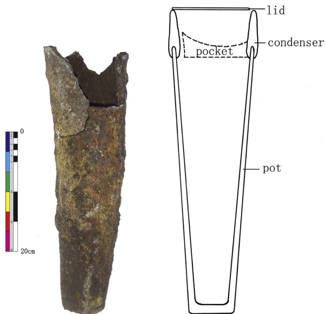
Fig. 2. Left: a nearly complete pot from Dafengmen collected during the 2004 field-work; right: Reconstruction of a Dafengmen retort, which was composed of pot, condenser, pocket and lid.
