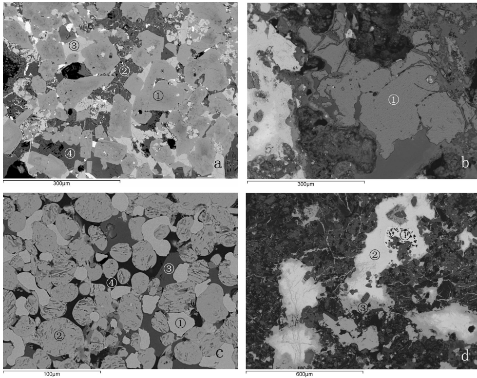
Fig. 6. BSE images of the slag samples from Dafengmen. a. barium feldspar (1), olivines (2)(3) and pyroxene (4) in SDB6; b. residual grains of zinc sulphides (1) in SDB9; c. metallic iron prills (1), zinc oxide (2), olivine (3) and pyroxene (4) in a large lump in SDB12; d. lead (1), lead oxide (2) and lead carbonates (3) in SDB9. The metallic lead particles are studded with silicon carbide grains (black) from the grinding papers used during sample preparation, due to the softness of lead metal.
