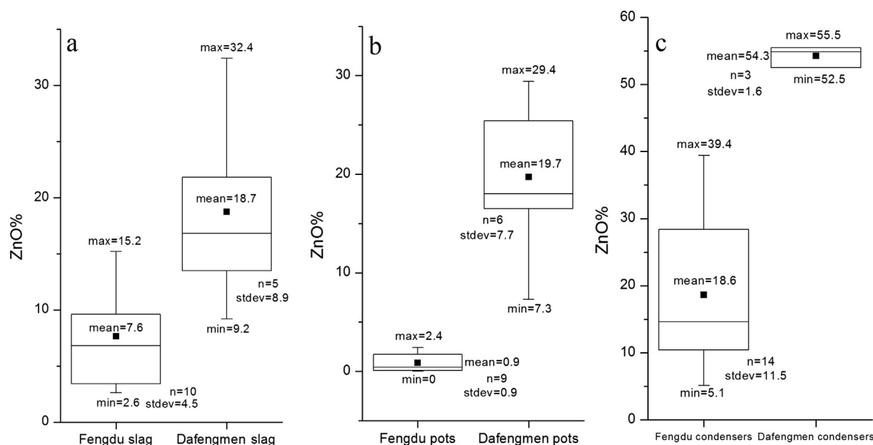
Fig. 11. Box and whisker charts of zinc oxide levels (wt%) of the slag (a), pot (b) and condenser (c) samples from the Fengdu sites and the Dafengmen site. All the zinc oxide values were bulk compositions of the slag, pots and condensers (max = maximum value; min = minimum value; mean = average value; n = number of samples; stdev = standard deviation).
