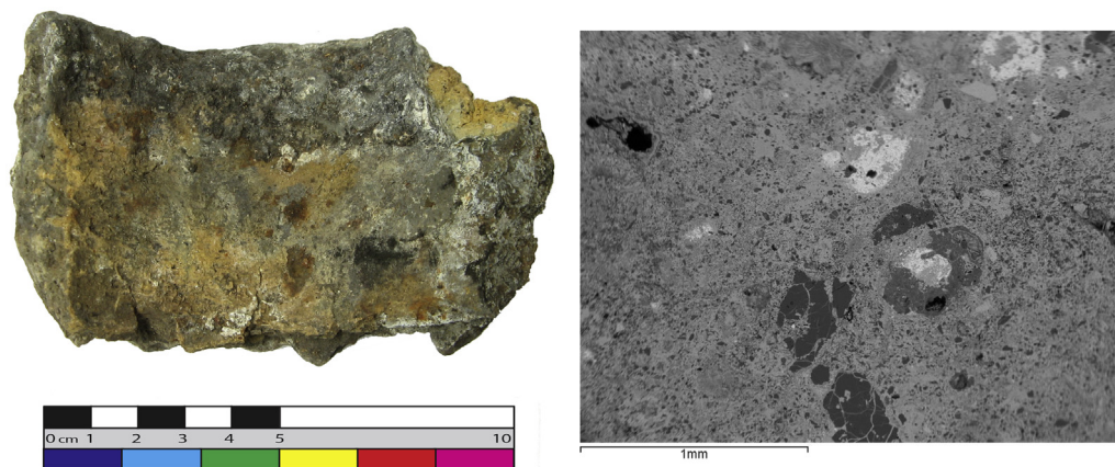
Fig. 4. Left: the internal surface of condenser SDT1; right: BSE image of the condenser fabric of SDT1, showing the heavily contaminated fabric and a few grains of inclusions.
