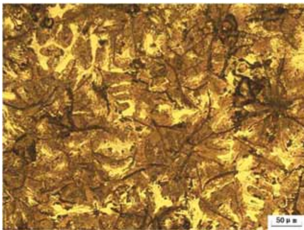
Figure 13: A grey cast iron object excavated from the Chengcun site, Fujian province.
