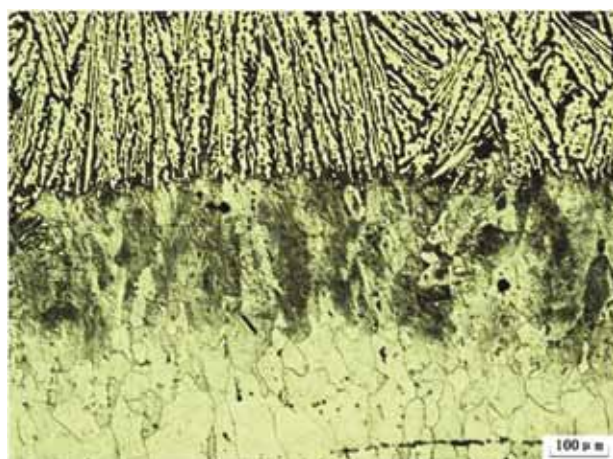
Figure 8: The microstructure of decarburised iron unearthed from the Yangying site, Hubei province.
