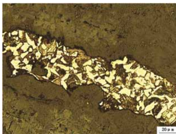
Figure 5: The microstructure of a carburised steel object excavated from the Ili Valley, Xinjiang.
