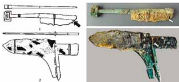
Figure 2: Two copper-iron bimetallic wares excavated from the Liangaicun site, Shaanxi province.
