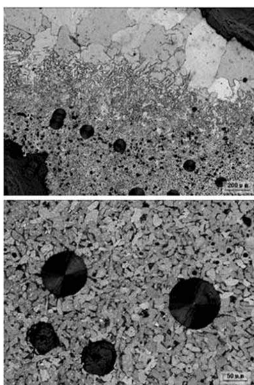
Figure 9: Spherical graphite in a malleable iron object excavated from Xinzhen, Henan province.
