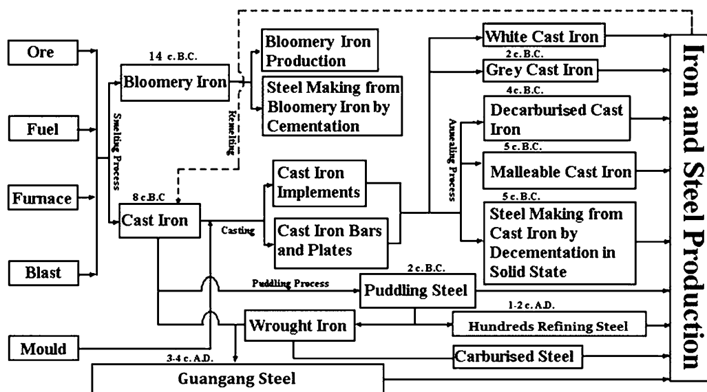
Figure 14: The system of iron and steel production techniques in ancient China.
