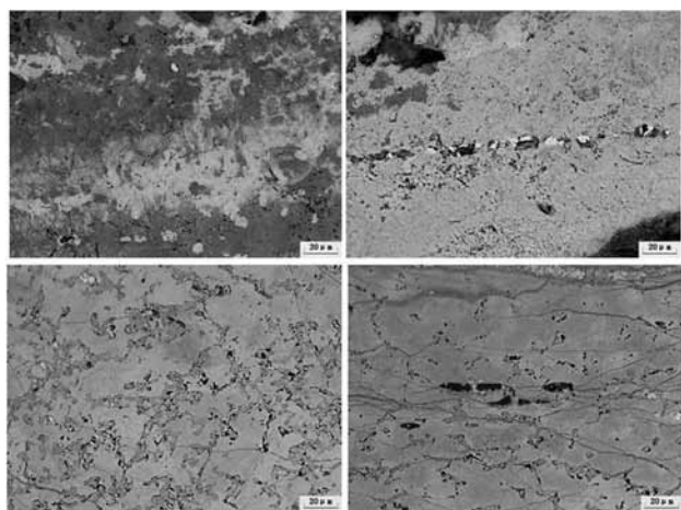
Figure 3: The microstructures of two copper-iron bimetallic wares excavated from the Liangaicun site, Shaanxi province.
