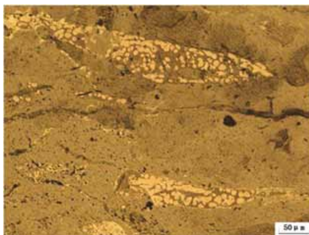
Figure 4: The microstructure of a bloomery iron object excavated from the Ili Valley, Xinjiang
