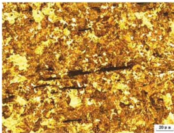
Figure 12: The microstructure of a puddling steel sword excavated from Suizhou, Hubei province.
